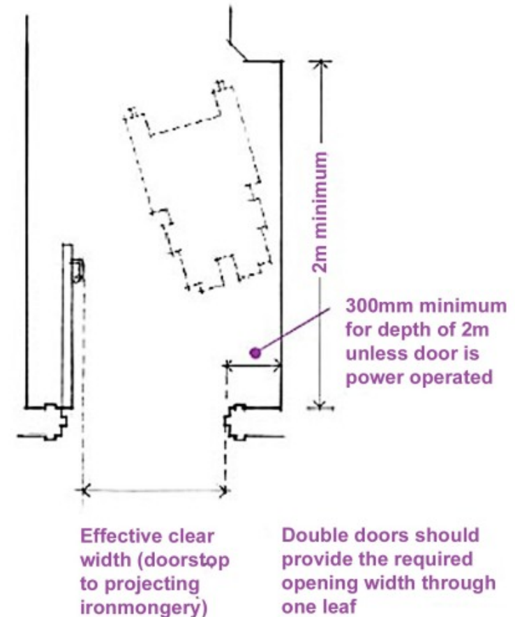
Figure 7 Effective clear width of door opening
