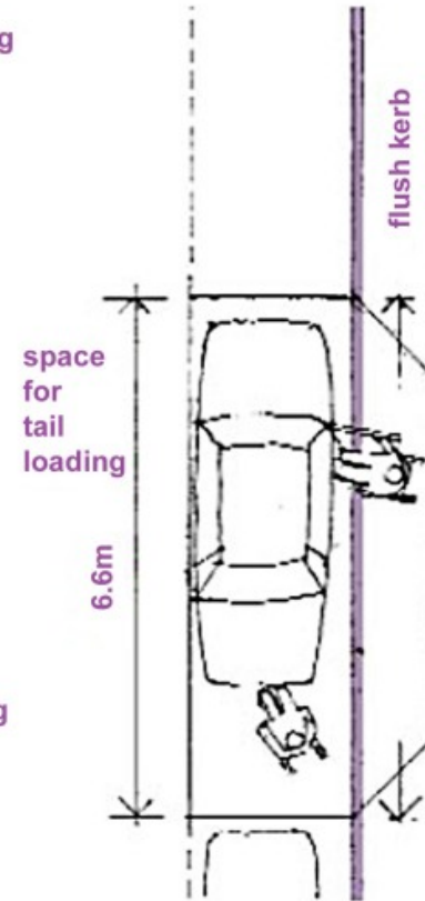
figure 06 On street parking bay
