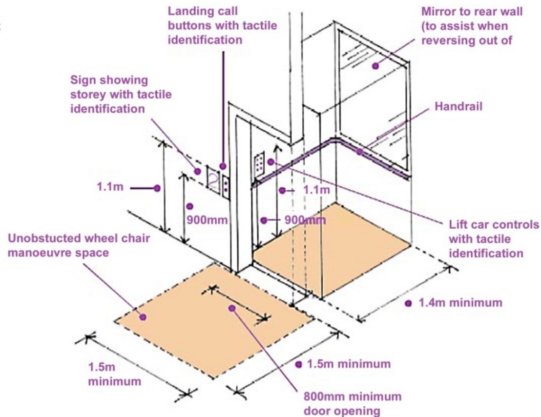
Figure 9 Passenger lift dimensions
